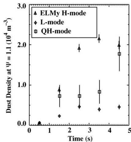
Fig. 2. Time dependence of dust density in the SOL ( \Psi = 1.1 ) for L, QH and ELMy H-mode.
