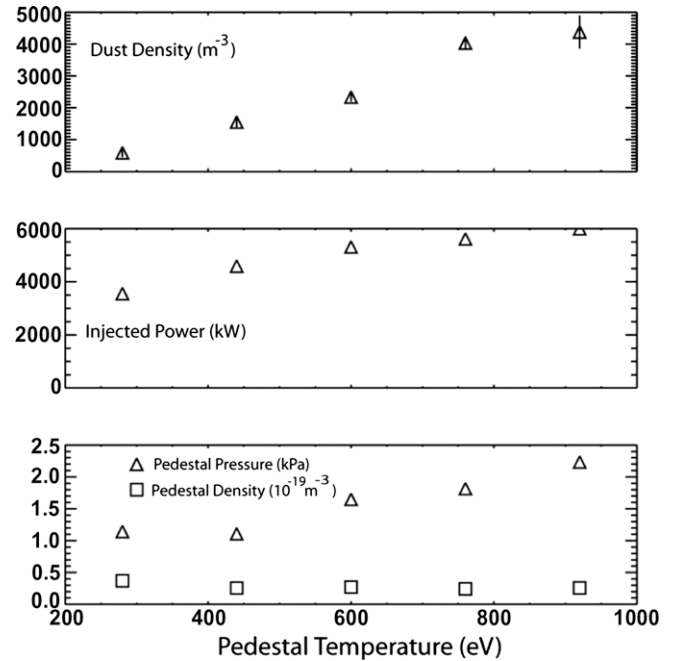
Fig. 3. Observed (a) dust density, (b) injected power and (c) pedestal pressure and density as a function of pedestal temperature.
