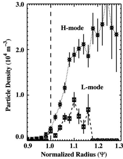
Fig. 1. Radial profile of dust density in the SOL for L- and H-mode.
