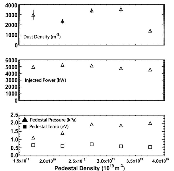
Fig. 4. Observed (a) dust density, (b) injected power and (c) pedestal pressure and temperature as a function of pedestal density.
